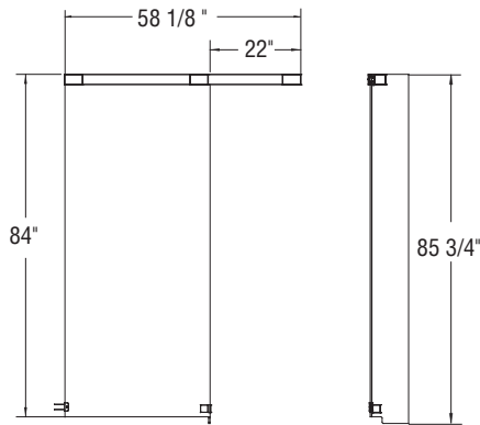
Walk-in glass enclosure
