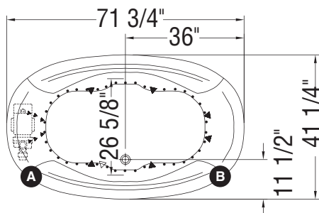
HYDROSENS, BACKMAX AND AIR SYSTEMS
