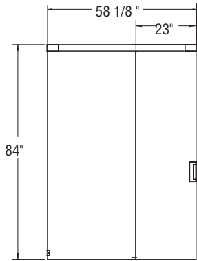
Glass enclosure with sliding door
