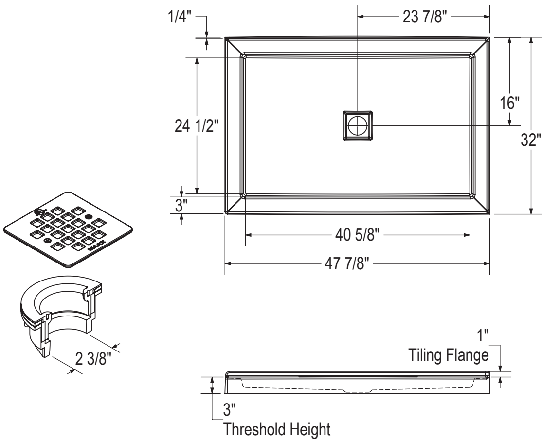
Right-Hand Tiling Flange (Shown)
