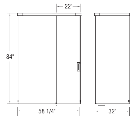
Glass enclosure with sliding door
