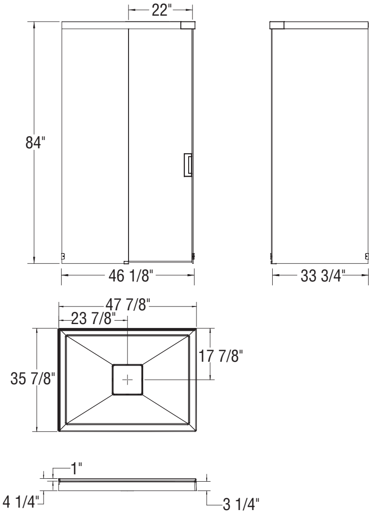
Right-hand door and left-hand base
