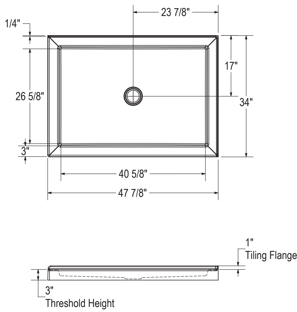
Right-Hand Tiling Flange (Shown)
