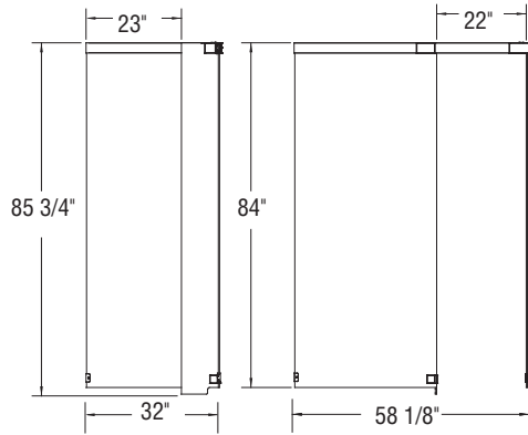
Walk-in glass enclosure
