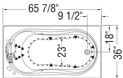
HYDROSENS, BACKMAX AND AIR SYSTEM
