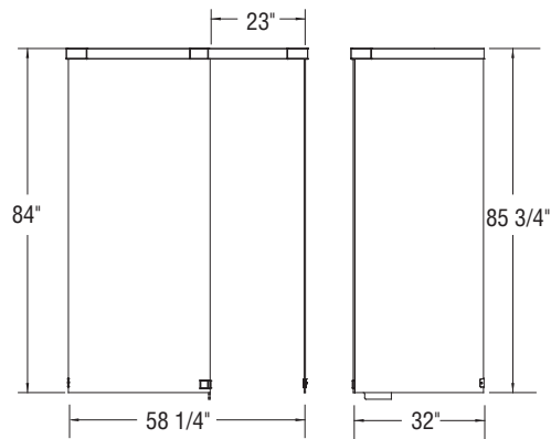
Walk-in glass enclosure
