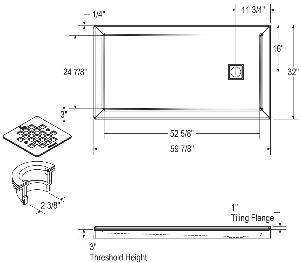
Right-Hand Drain & Tiling Flange (Shown)
