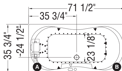
HYDROSENS, BACKMAX AND AIR SYSTEM
