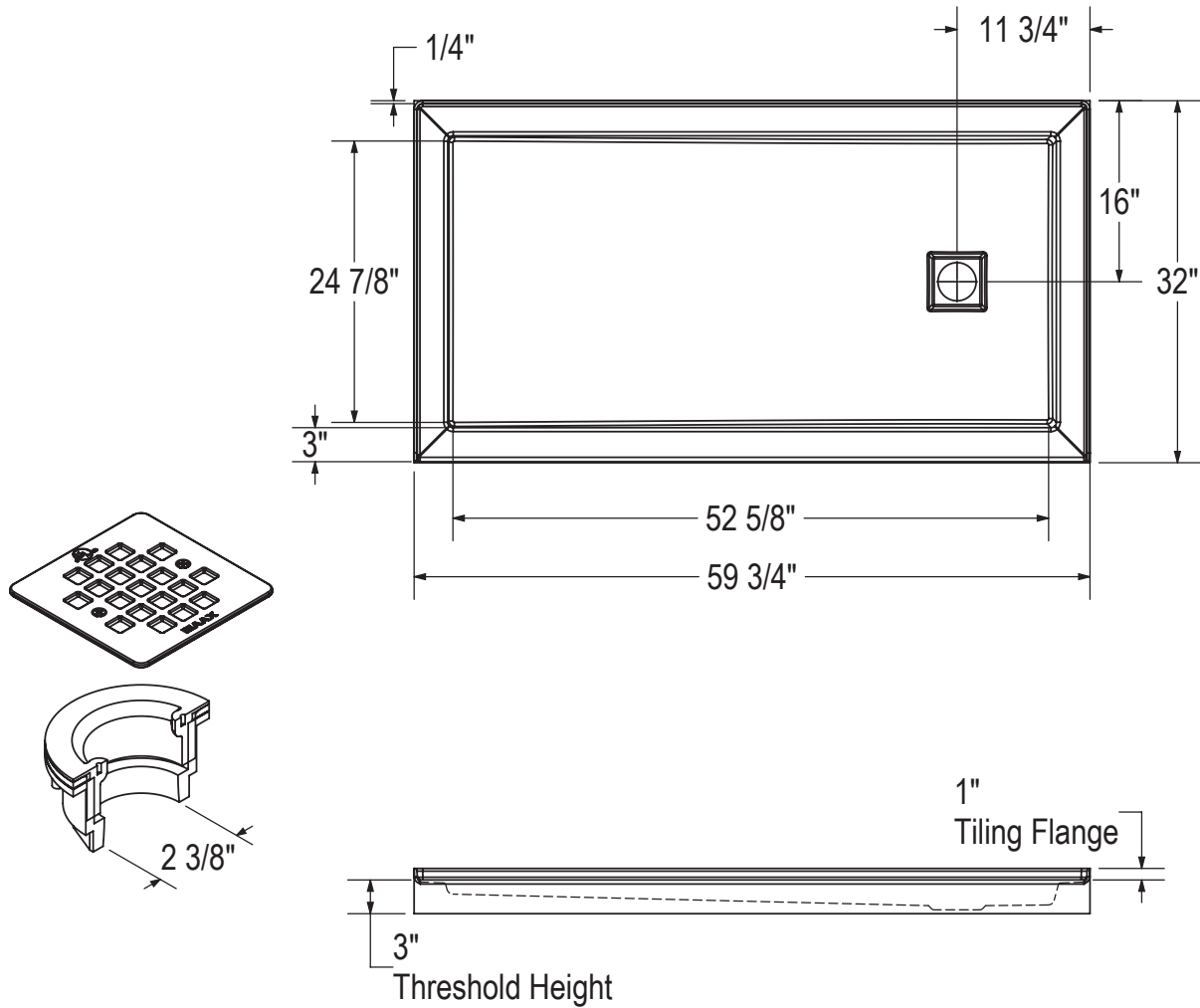
Right-Hand Drain (Shown)
