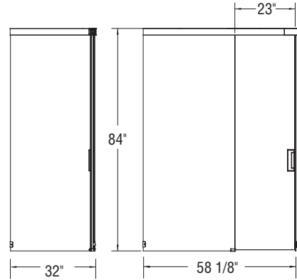
Glass enclosure with sliding door
